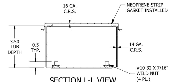
SECTION L-L VIEW (INSIDE TOP OF ENCL.)
