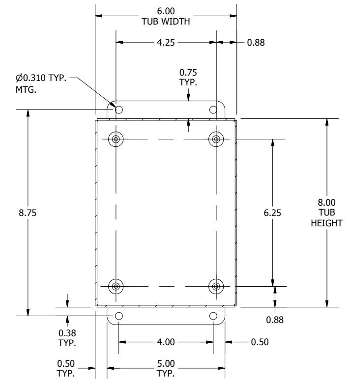
SECTION K-K VIEW (INSIDE BACK OF ENCL.)
