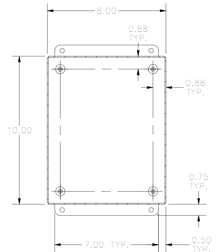
SECTION K-K (INSIDE BACK OF ENCLOSURE)
