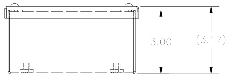
BOTTOM VIEW
