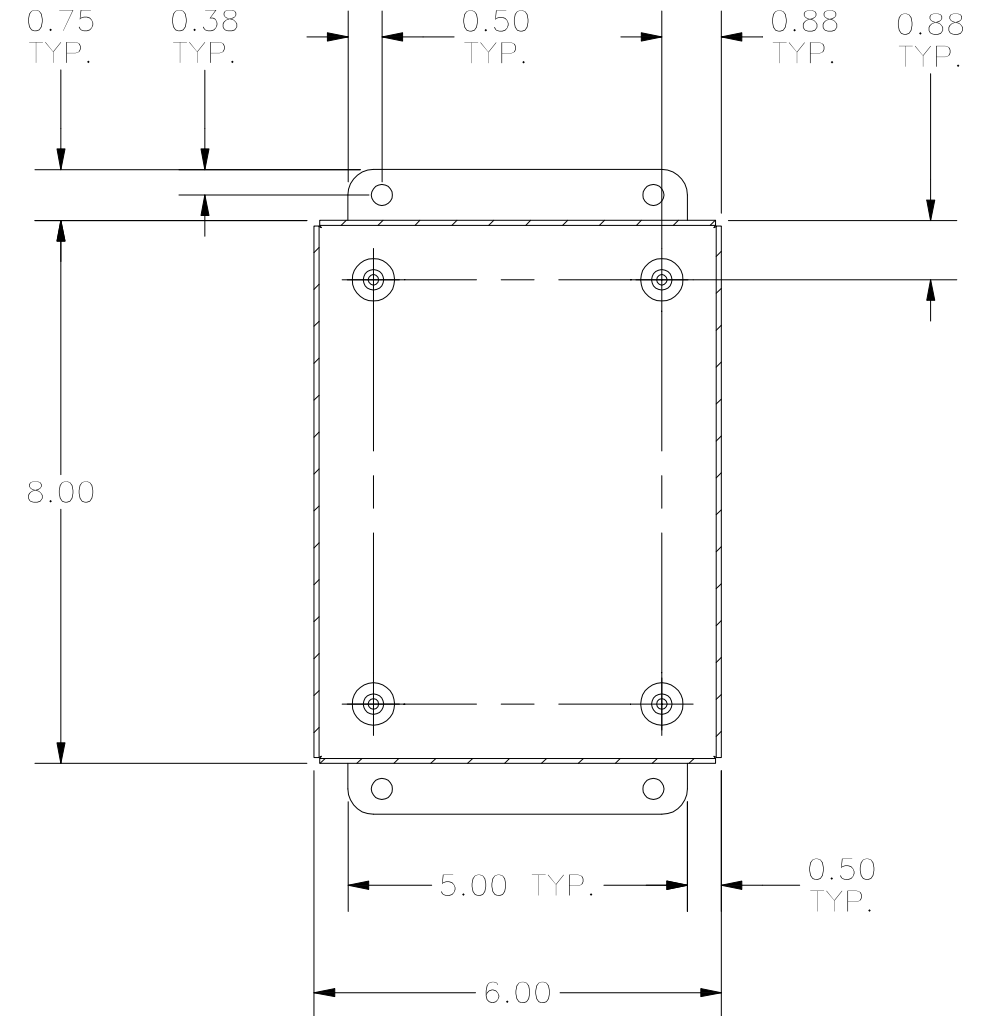
SECTION K-K (INSIDE BACK OF ENCLOSURE)
