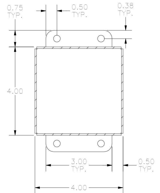
SECTION K-K (INSIDE BACK OF ENCLOSURE)
