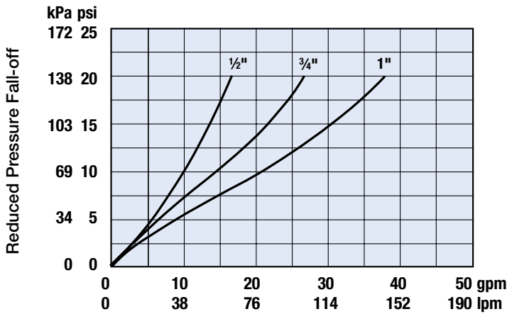
Sizes 1/2", 3/4", 1" (15, 20, 25mm)
