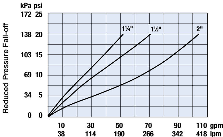
Sizes 1 1/4", 1 1/2", 2" (32, 40, 50mm)
