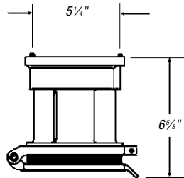
200A MaxGard® inlets with disconnects
