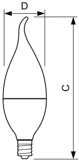
LED 4.5-40W E12 BA12 CL DIM
