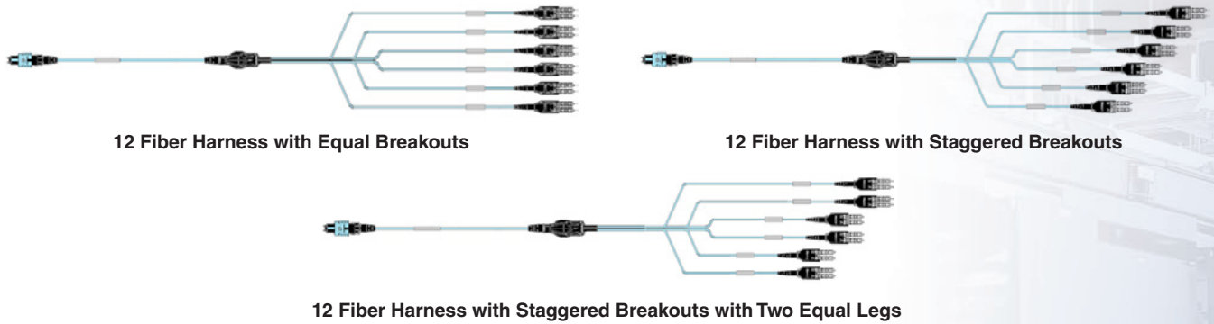
Figure 4 – Harness Configurations
