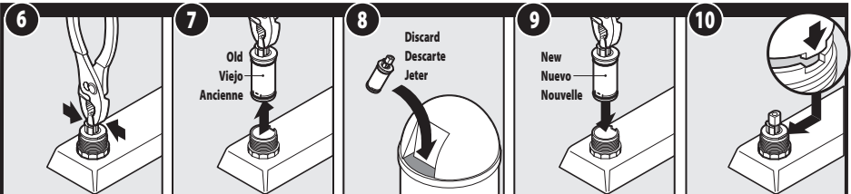
REASSEMBLY, REVERSE Steps 5-1
