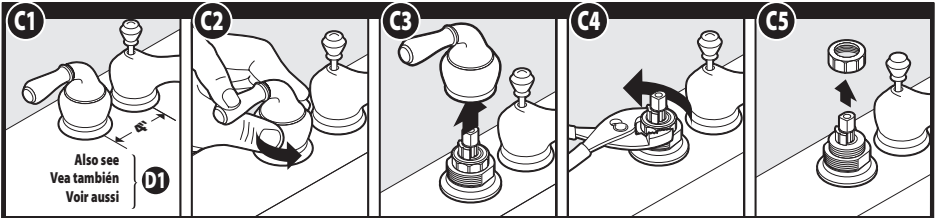
CARTRIDGE REMOVAL/INSTALLATION
