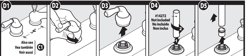
REASSEMBLY, REVERSE Steps D7-D1
