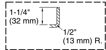
Integral Flange Detail
