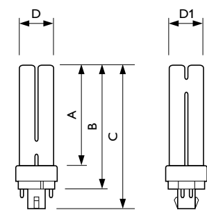
PL-C 18W/830/4P
