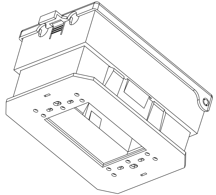
ISOMETRIC VIEW
