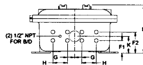
Panel E – End View
