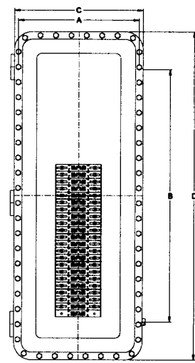
Panel H – Front View
