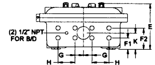
Panel C – End View
