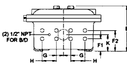
Panel D – End View
