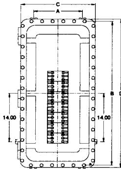
Panel D – Front View
