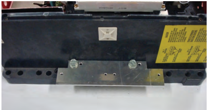
Figure 8. C/D Terminal Block Mounting Plate Installed on the Base.
