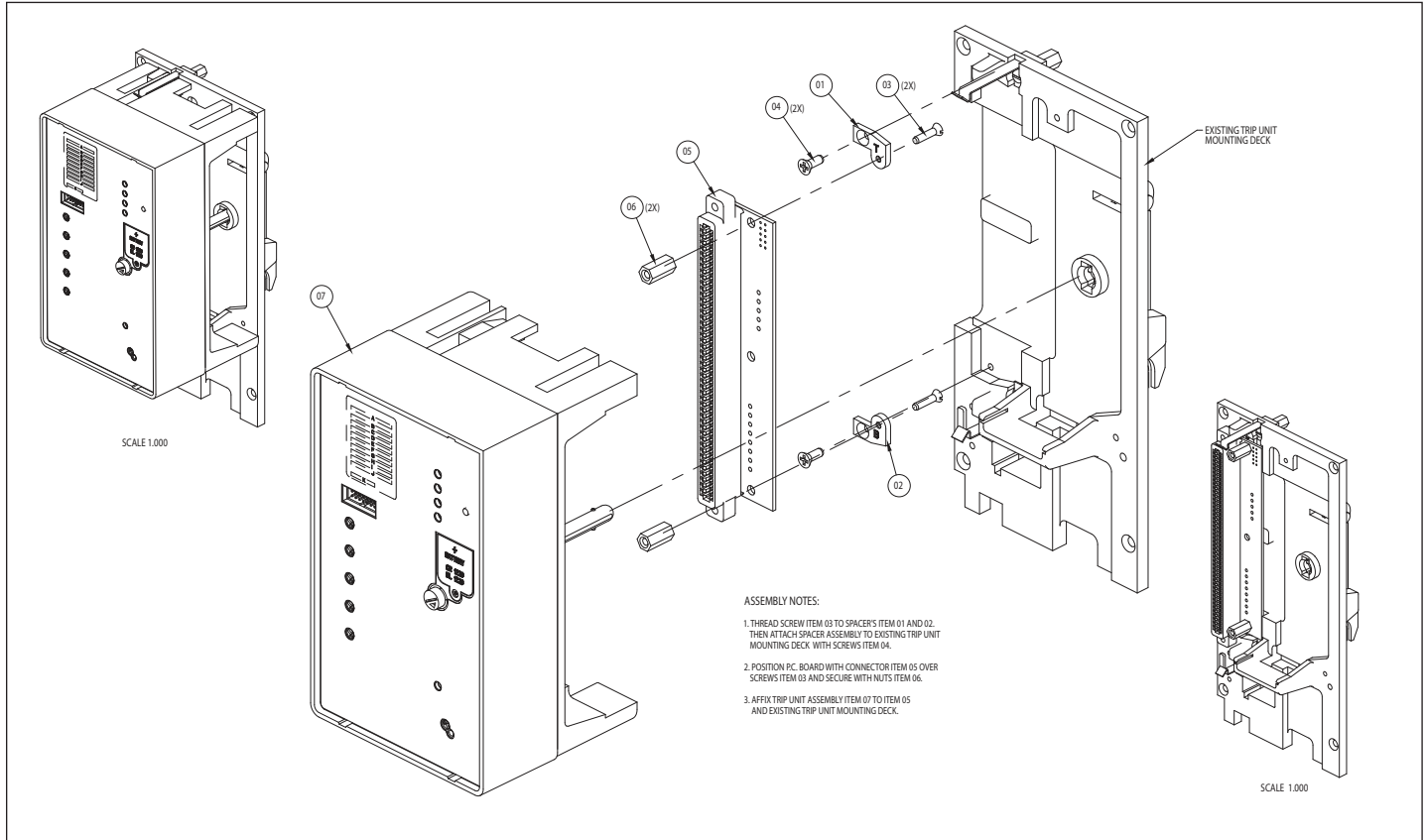
Figure 28. Drawing #6D32435.
