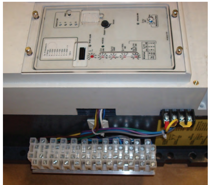
Figure 24. Breaker with Trip Unit Cover Installed (Note: Retrofit Label Not Shown in Photo).
