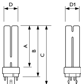
PL-C XEW 18W/835/4P ALTO 14W
