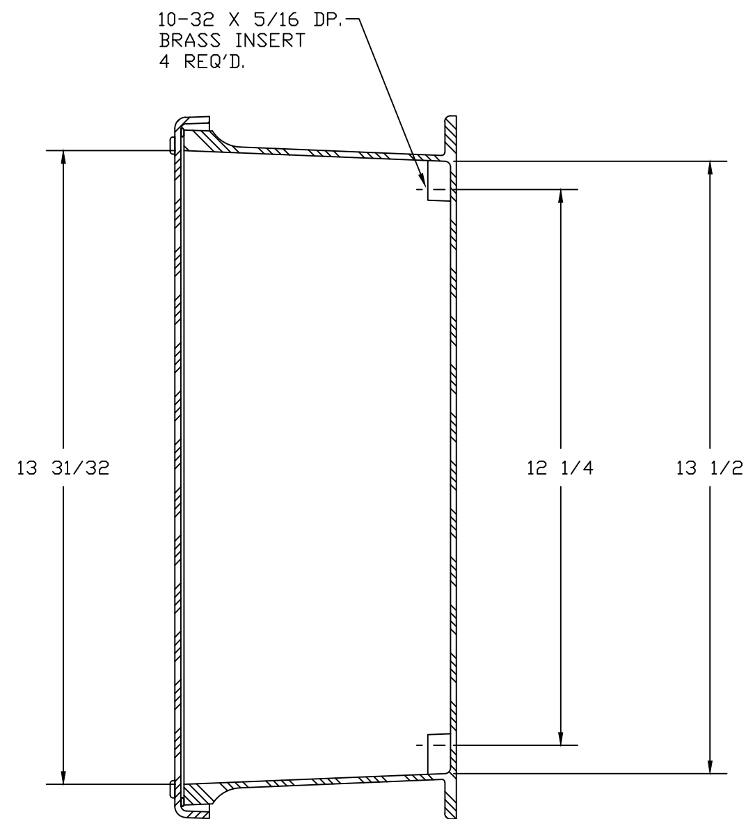
SECTION B-B
