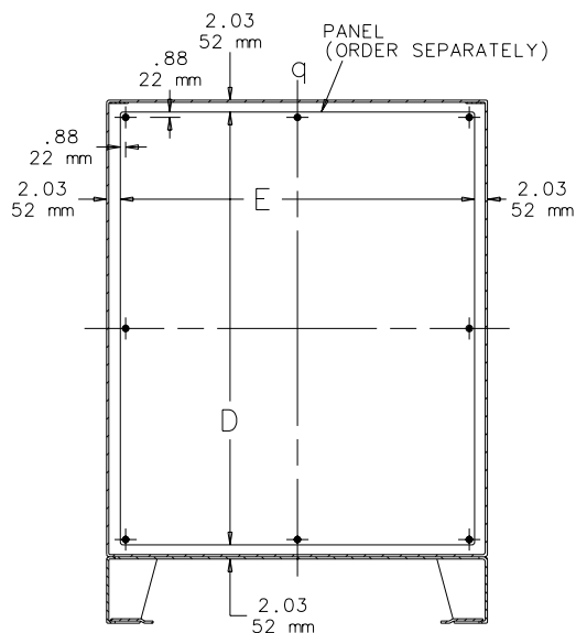
SECTION Y-Y
