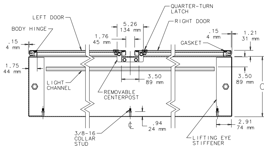
SECTION X-X
