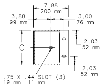
SECTION W-W
