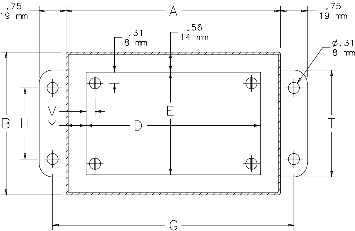
SECTION Y-Y
