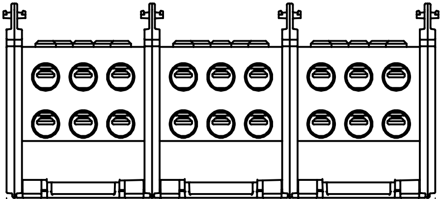
3.25 ONE POLE [83] 6.17 TWO POLE [157] 9.09 THREE POLE [231] TAP SIDE
