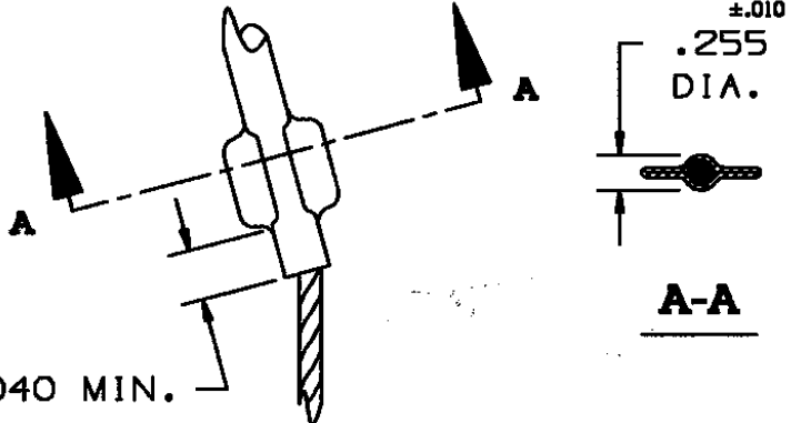
CRIMP DETAIL 2 PL.
