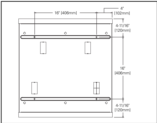
Diagram 1: Hole Mounting
