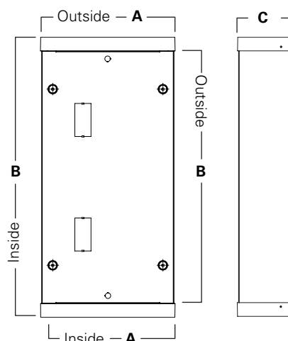
Diagram 2: Access Plate Location
