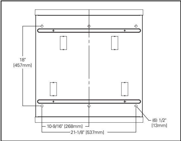
Diagram 3: Pendant Mounting
