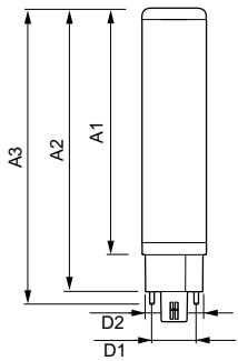
LEDtube 100mm 8.5W/830
