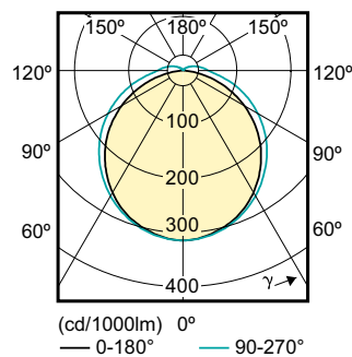
LED InstantFit PL-C/T 100mm 8.5 W
