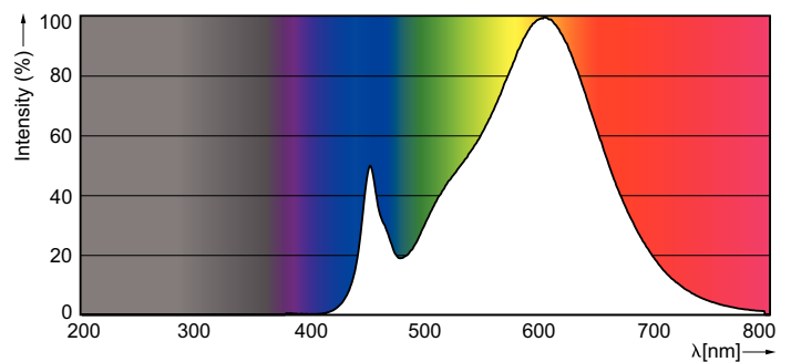
LED InstantFit PL-C/T 100mm 8.5 W /830
