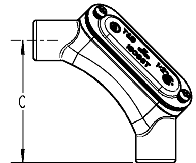
ASSEMBLED CONDUIT BODY IS SHOWN
