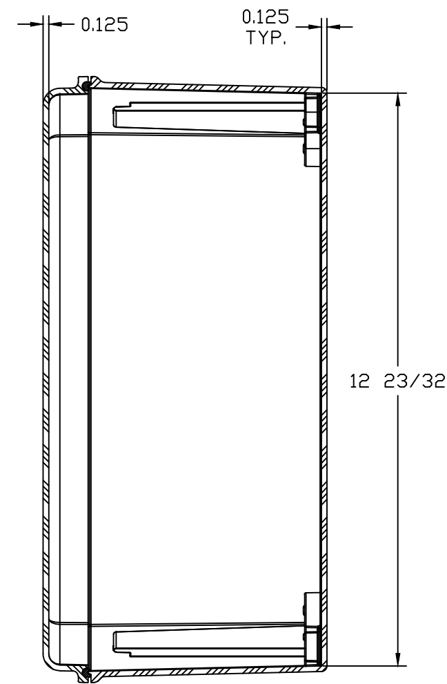
SECTION B-B
