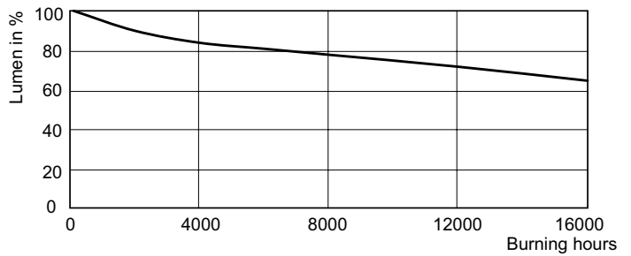
ALTO Elite PAR38 70 W, 100 W /830
