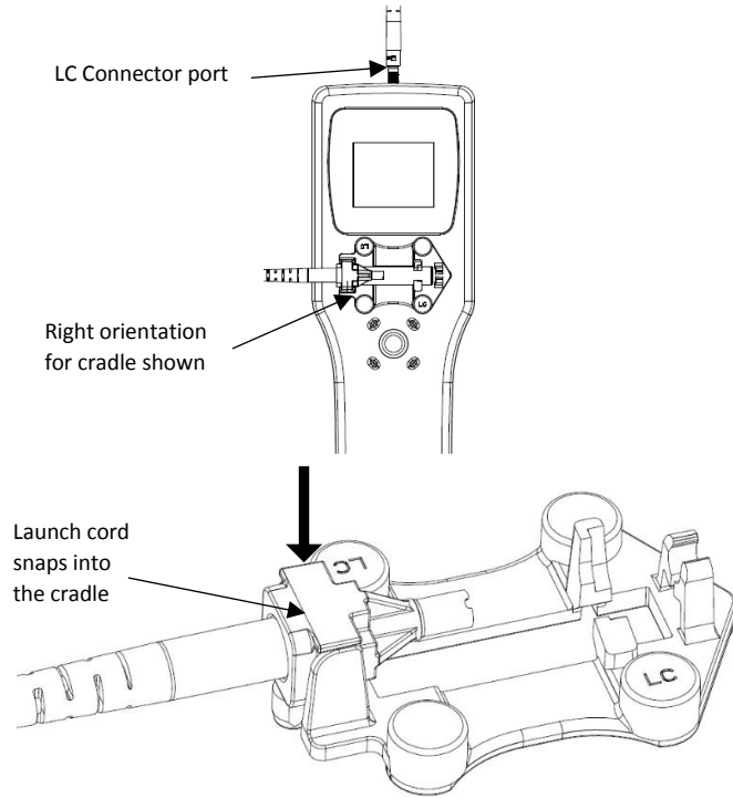
Right Orientation for the cradle Left Orientation for the cradle
