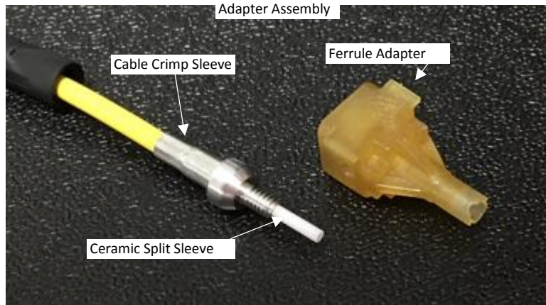
LC Launch Cord Ferrule Adapter
