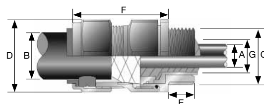
Dimensions in Millimeters (Inches)
