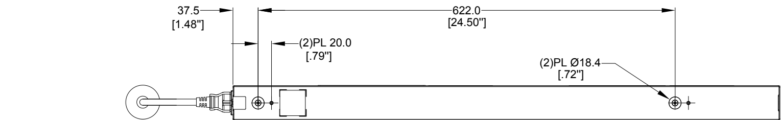
REAR VIEW
