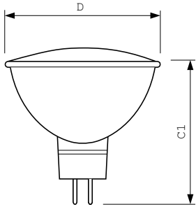
MLES Alu 35W GU5.3 12V MR16 24D
