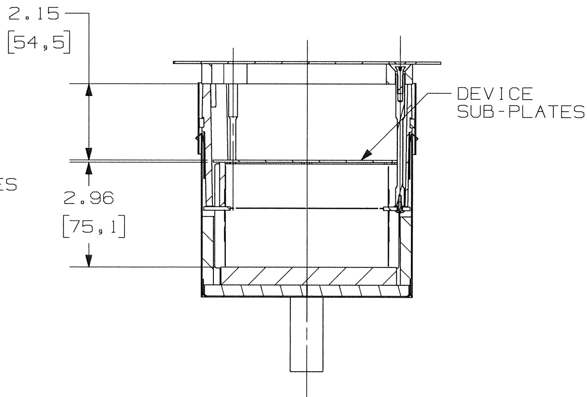
SECTION B-B
