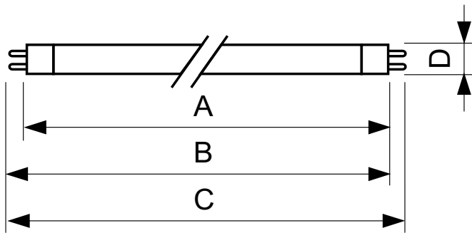
TL5 HE F14T5/841 HE Alto
