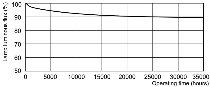
MASTER TL5 HE Lumen Maintenance 3 h + 12 h cycle
