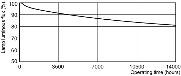
Lumen Maintenance 3 h + 12 h cycle
