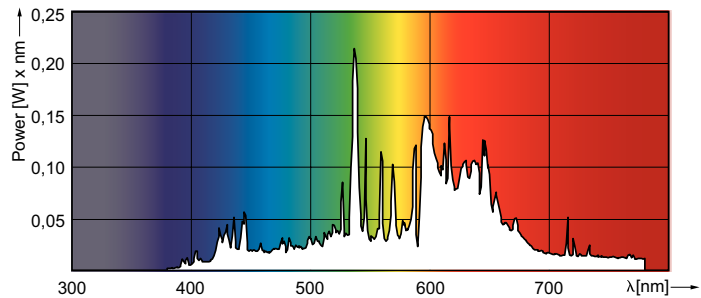
CDM-R Elite 35W /930 PAR30L
