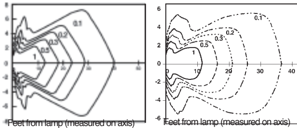
6 volt, 7.2 watt SBT Lamp
