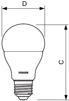
Bulb A19 120V 6.5W 450lm 2700K E26 Dim
