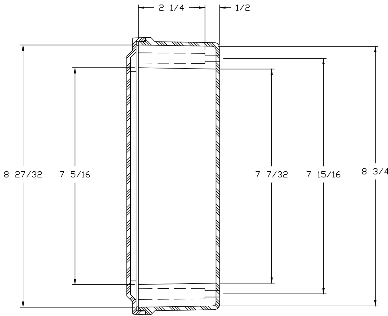
SECTION B-B
