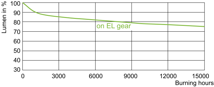
CDM-TC 20W Lumen Maintenance /830
