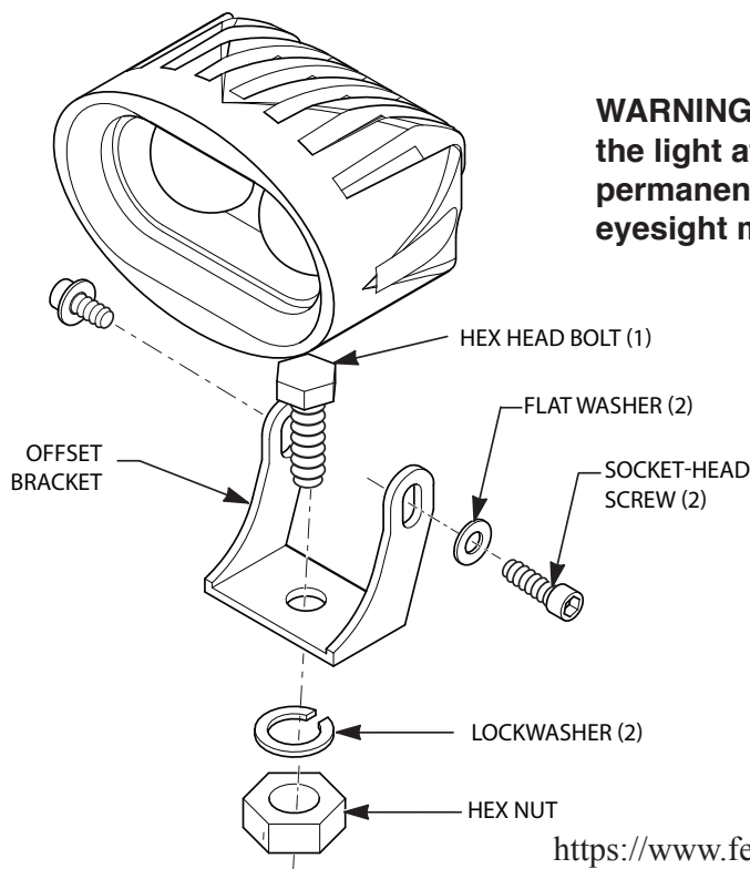
Exploded view of the COMFL1 with mounting hardware
