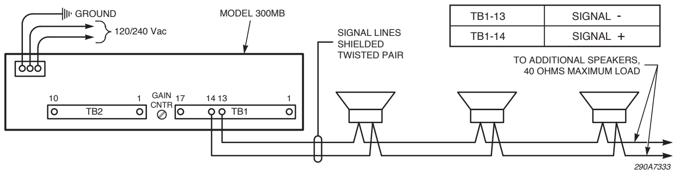
Figure 8 Model 300MB with 25 Vrms connections
