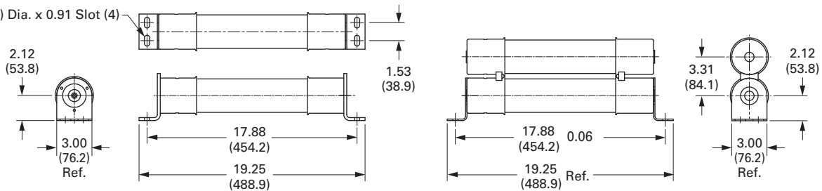
Type 5BCLS and 7BCLS Fuses
