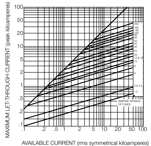
Figure 7. Maximum let-through current for NX current-limiting fuses – 8.3, 15.5 and 23 kV.
