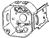
1-1/2" Deep JB Bracket set flush; Gauging Notches 3/8" & 1/2"
