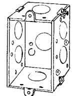
2-1/2" Deep, Gangable; Four nail holes, each side; Side leveling bosses
