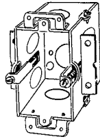
2-1/2" Deep, Gangable Old work -support clamps Plaster ears
