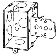
2-1/2" Deep, Gangable Stud NL bracket set back 1/2"
