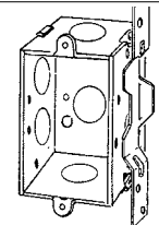
2-1/2" Deep, Gangable; Plain vertical bracket set back 3/4"
