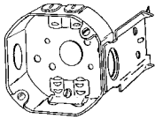
2-1/8" Deep JB Bracket set back 1"; Gauging Notches 3/8" & 1/2"
