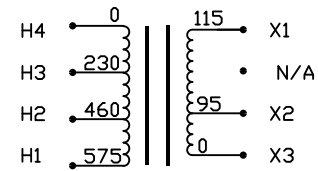
CONNECTION DIAGRAM
