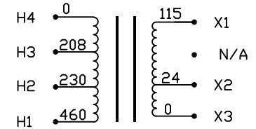
CONNECTION DIAGRAM
