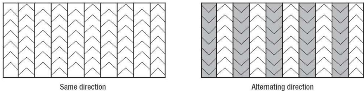
Embossed Grain Pattern and Streaking Pattern Orientation During Installation
