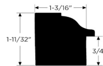
Back Band WPVCM-6931 1202943 - 16' 1418318 - 12' ●
