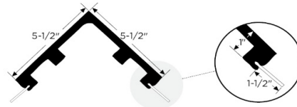
Outside Corner w/ Flex Nail Fin WPVCM-OCPF 1418310 - 20'
