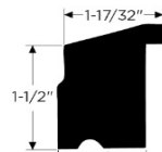
Sub Sill Nose
