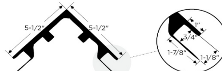
Outside Corner w/ J and Nail Fin
