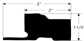
Brick Mould w/ Fin
