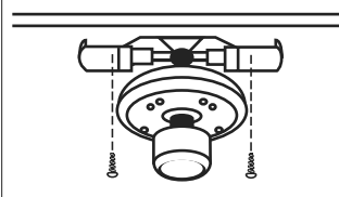
FIGURE - 4 DOWNROD FANS ONLY
