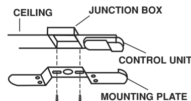
FIGURE - 5 FLUSHMOUNT FANS ONLY
