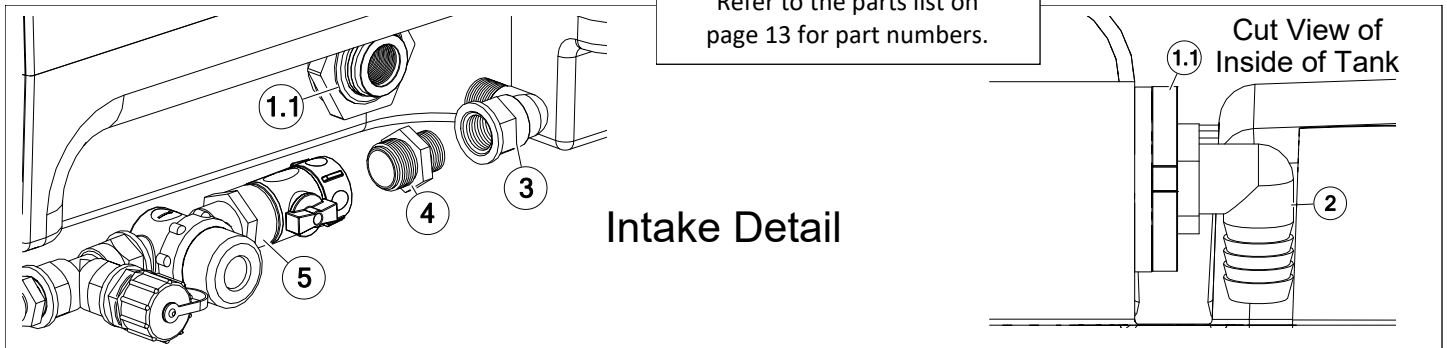
Boomless "Wet" Boom Assembly Exploded View/Parts List (5275260)
