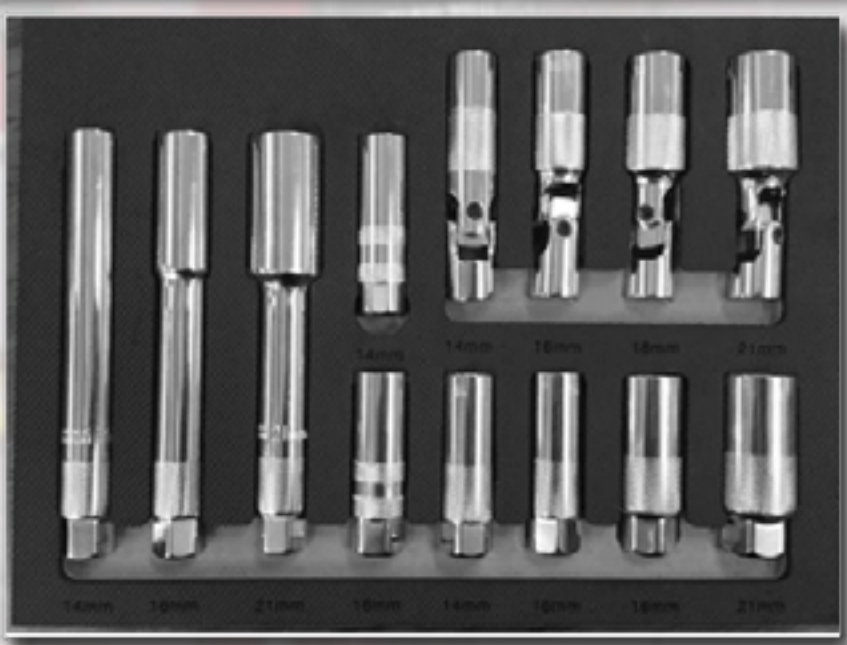
SPM100 Spark Plug Master Set Shown on Page 24
