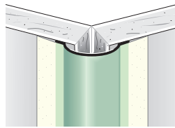
USG Beadex™ Brand Paper-Faced Metal Corner Bead 1/2" Bullnose Outside Corner (Baby Bull®)
