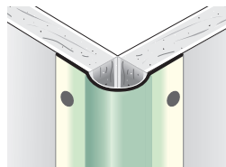
USG Beadex™ Brand Paper-Faced Metal Corner Bead 3/4" Bullnose Inside Corner (SLIC)
