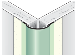
USG Beadex™ Brand Paper-Faced Metal Corner Bead 3/4" Bullnose Outside Corner (SLOC)
